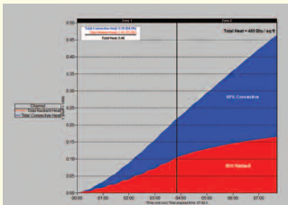
Heat Flux
